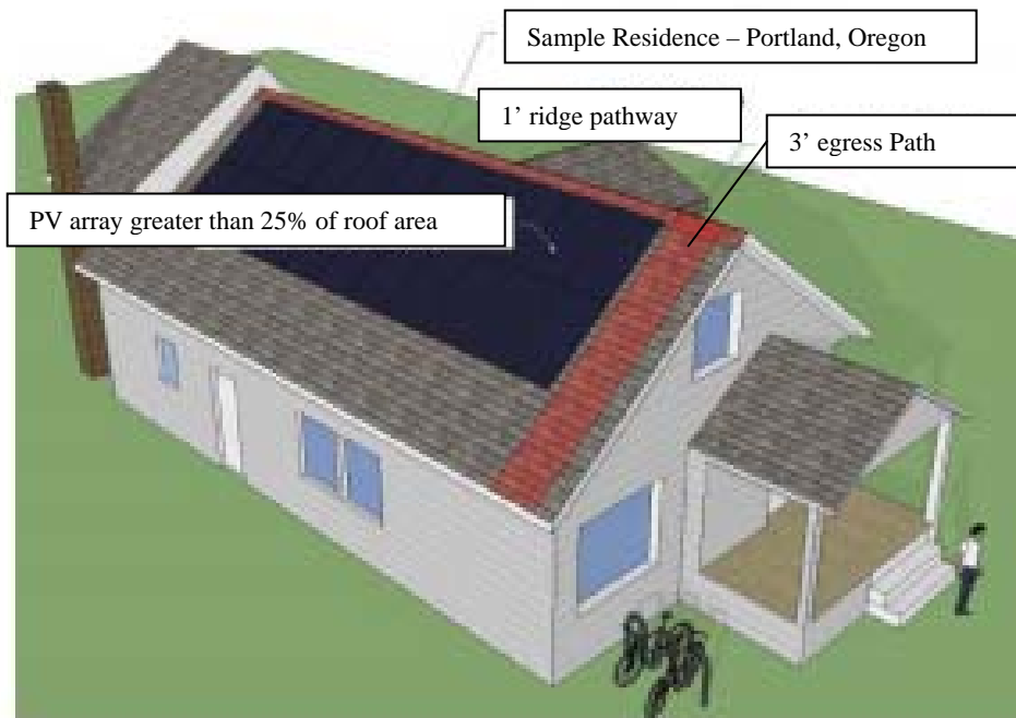
FIGURE 309.1 PANEL PATHWAY LOCATIONS
