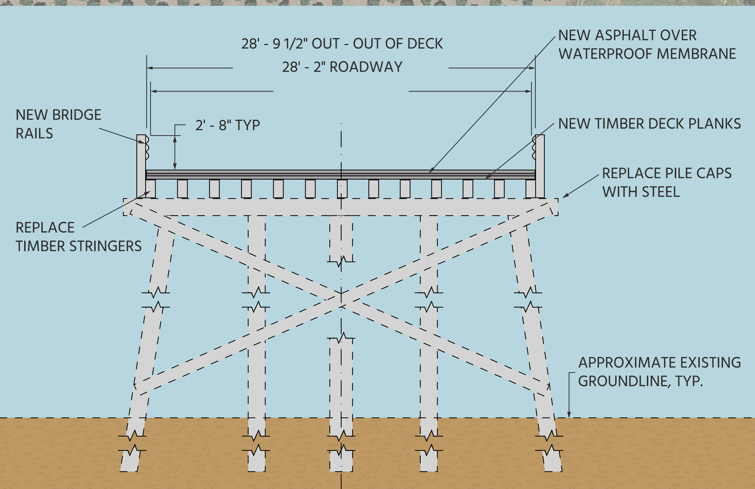
TYPICAL BENT SECTION
