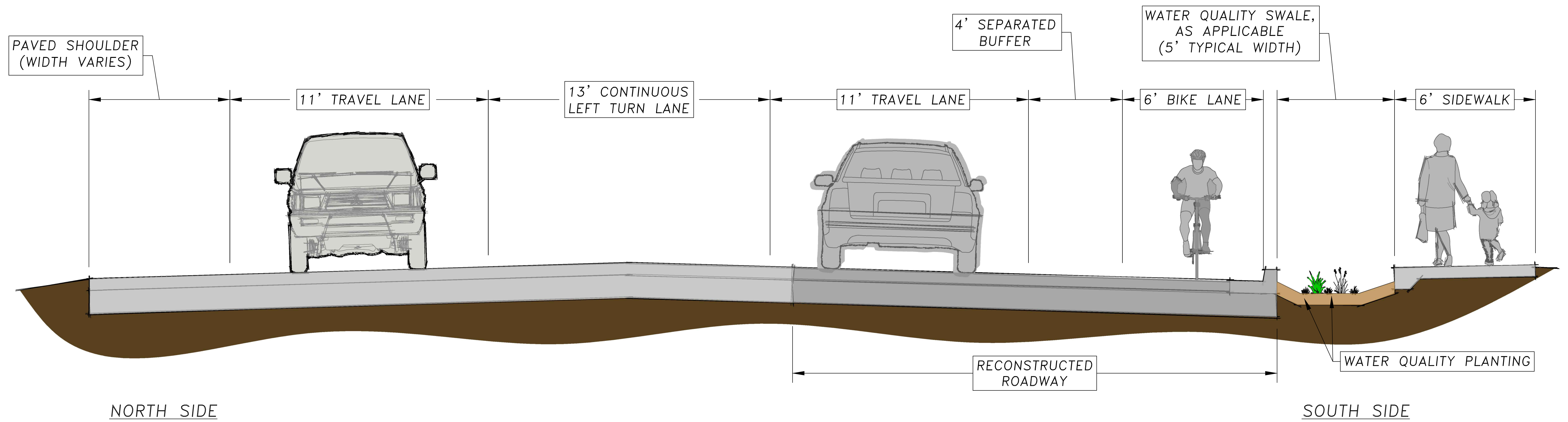
① TYPICAL SECTION WITH LANDSCAPED BUFFER SCALE: NTS
