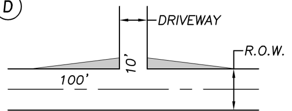
DRIVEWAY/COLLECTOR OR ARTERIAL
