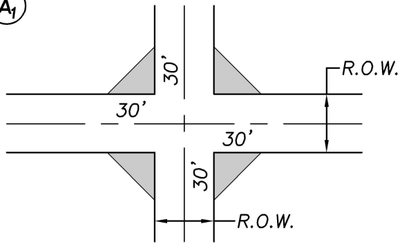
LOCAL/LOCAL (NO STOP)
