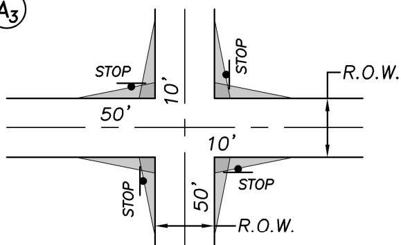
LOCAL/LOCAL (FOUR-WAY STOP)
