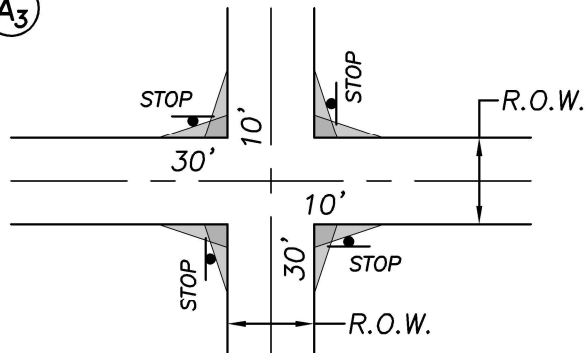
LOCAL/LOCAL (FOUR-WAY STOP)
