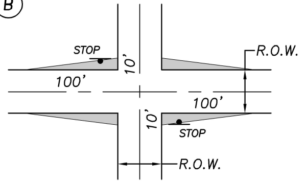
LOCAL/COLLECTOR OR ARTERIAL
