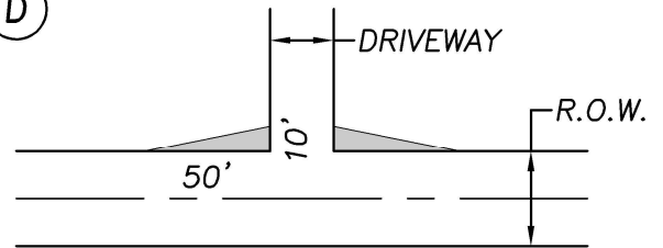
DRIVEWAY/COLLECTOR OR ARTERIAL
