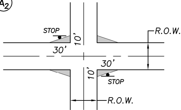
LOCAL/LOCAL (TWO-WAY STOP)
