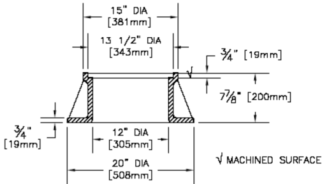
FRAME SECTION
