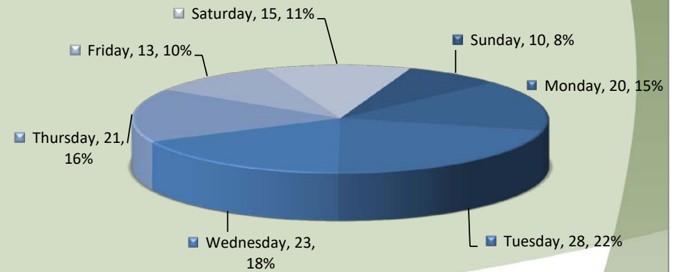
Calls for Service by Day of Week Jefferson - October 2019
