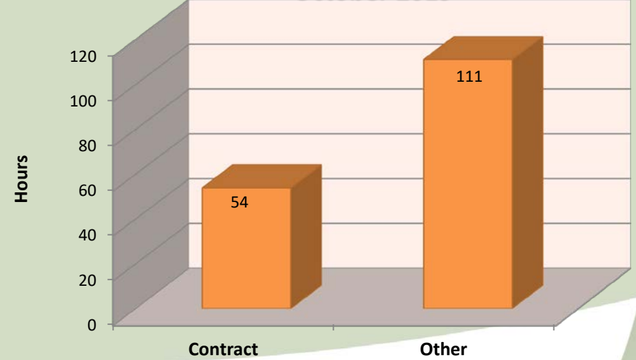
City of Jefferson Total Call Length October 2019
