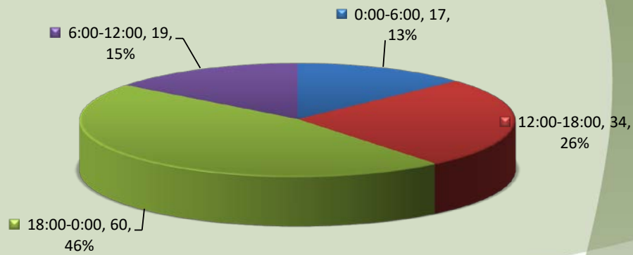
Calls for Service by Hours Range Jefferson - October 2019
