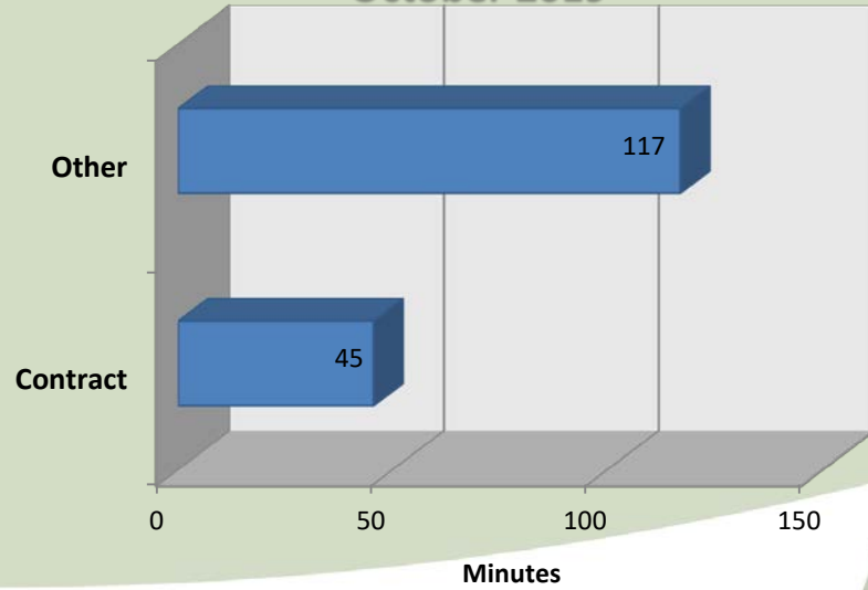
City of Jefferson Average Call Length October 2019
