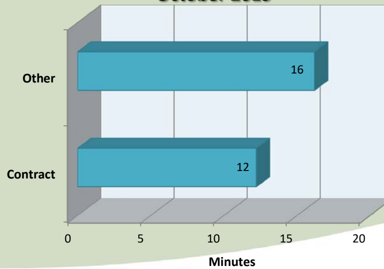
City of Jefferson Average Call Arrival Time (Traffic Removed) October 2019
