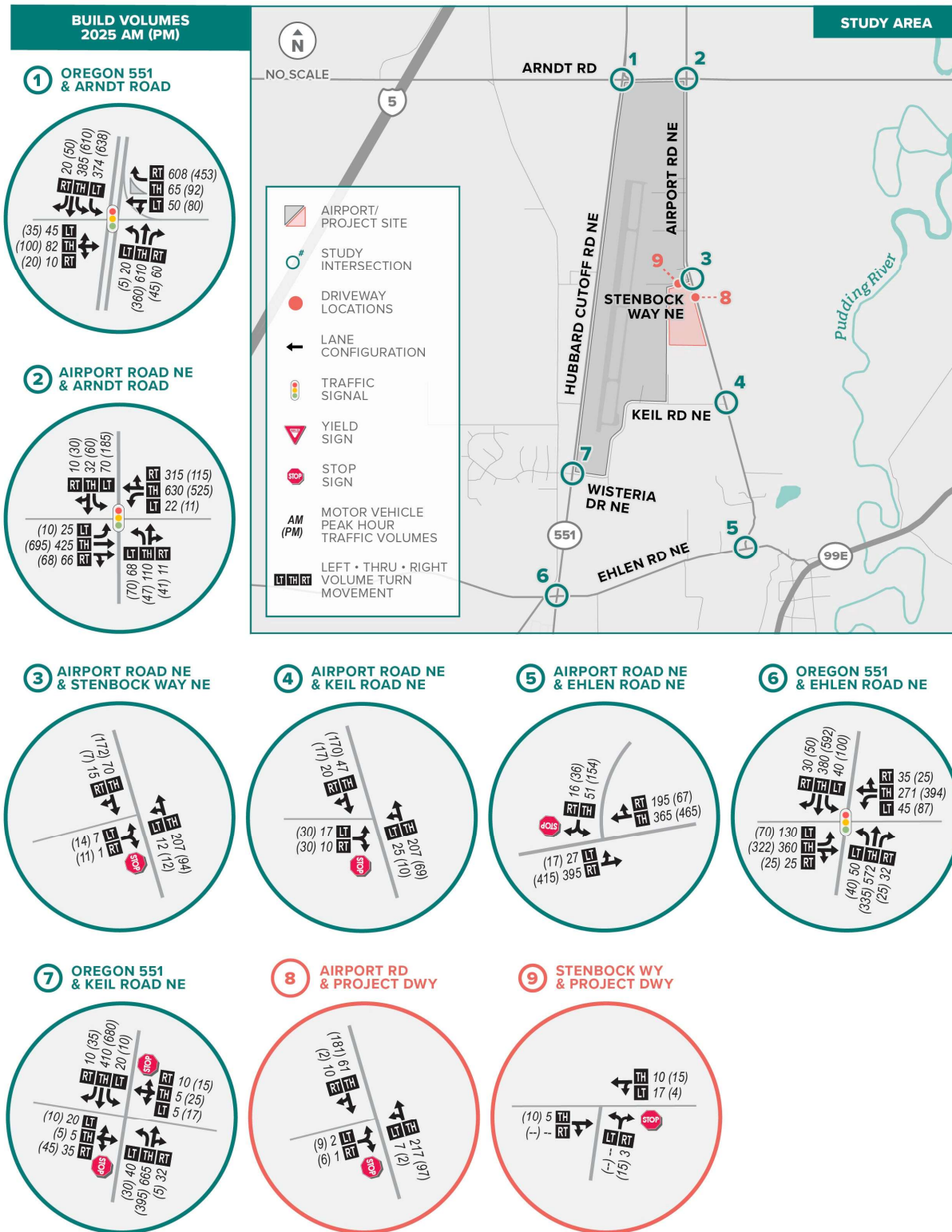
FIGURE 6: 2025 BUILD TRAFFIC VOLUMES
