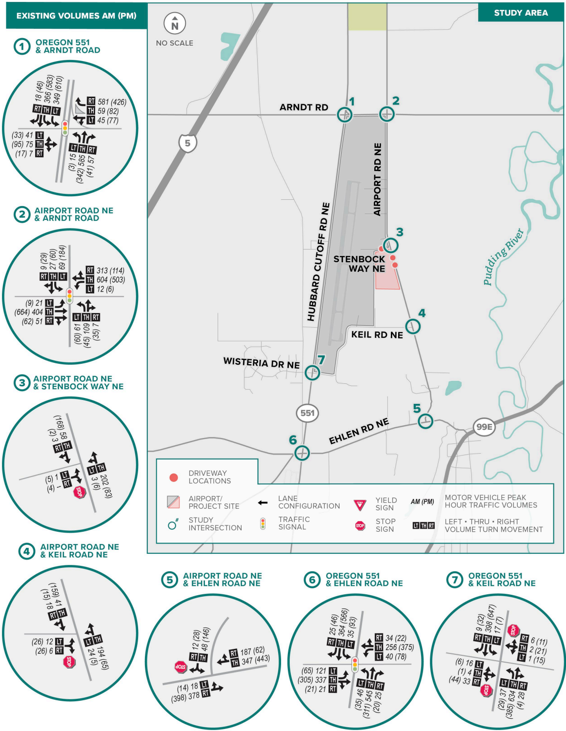
FIGURE 2: 2023 EXISTING CONDITIONS TRAFFIC VOLUMES
