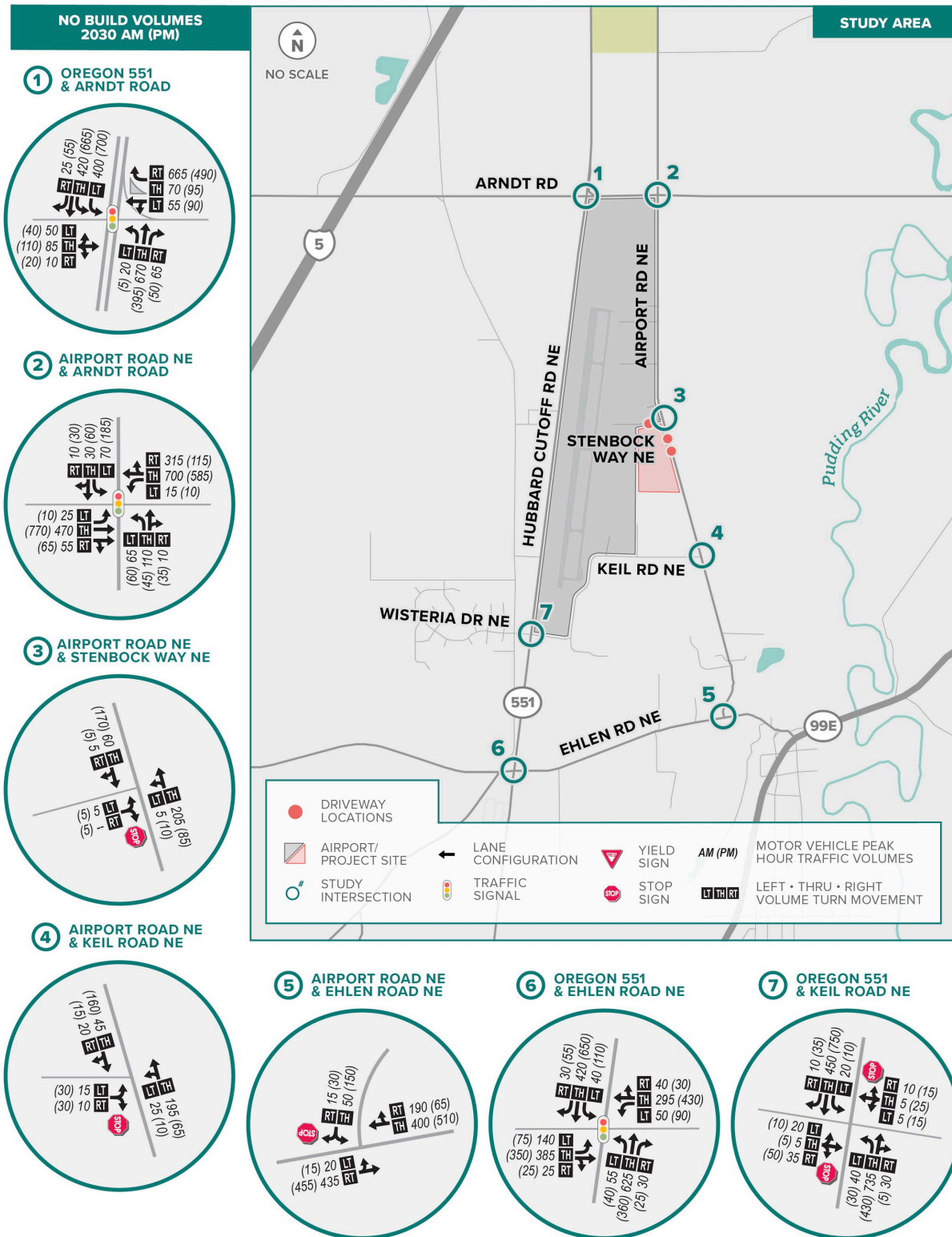
FIGURE 7: 2030 NO BUILD TRAFFIC VOLUMES
