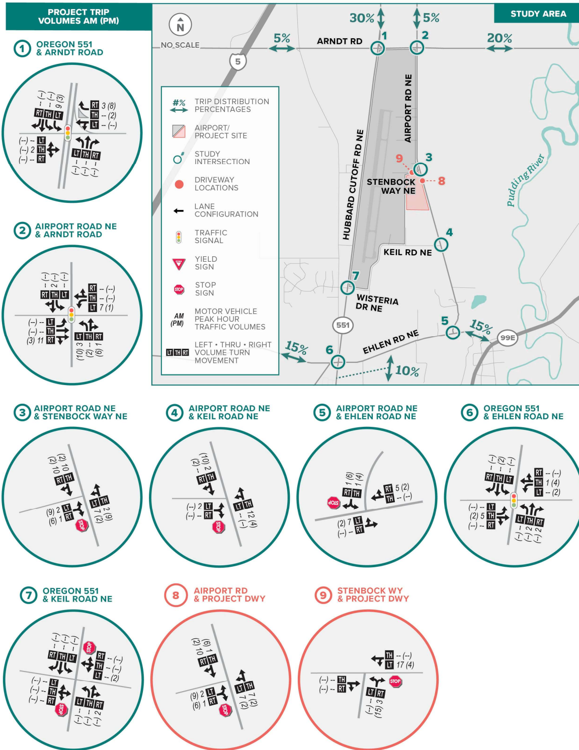
FIGURE 4: PROJECT TRIPS AND TRIP DISTRIBUTION
