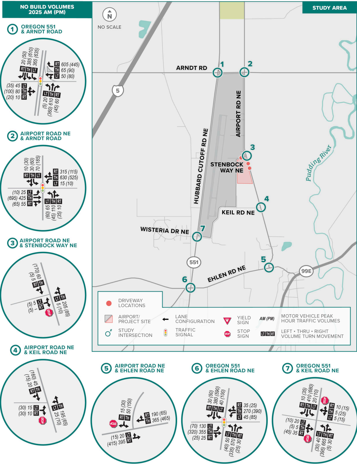
FIGURE 5: 2025 NO BUILD TRAFFIC VOLUMES
