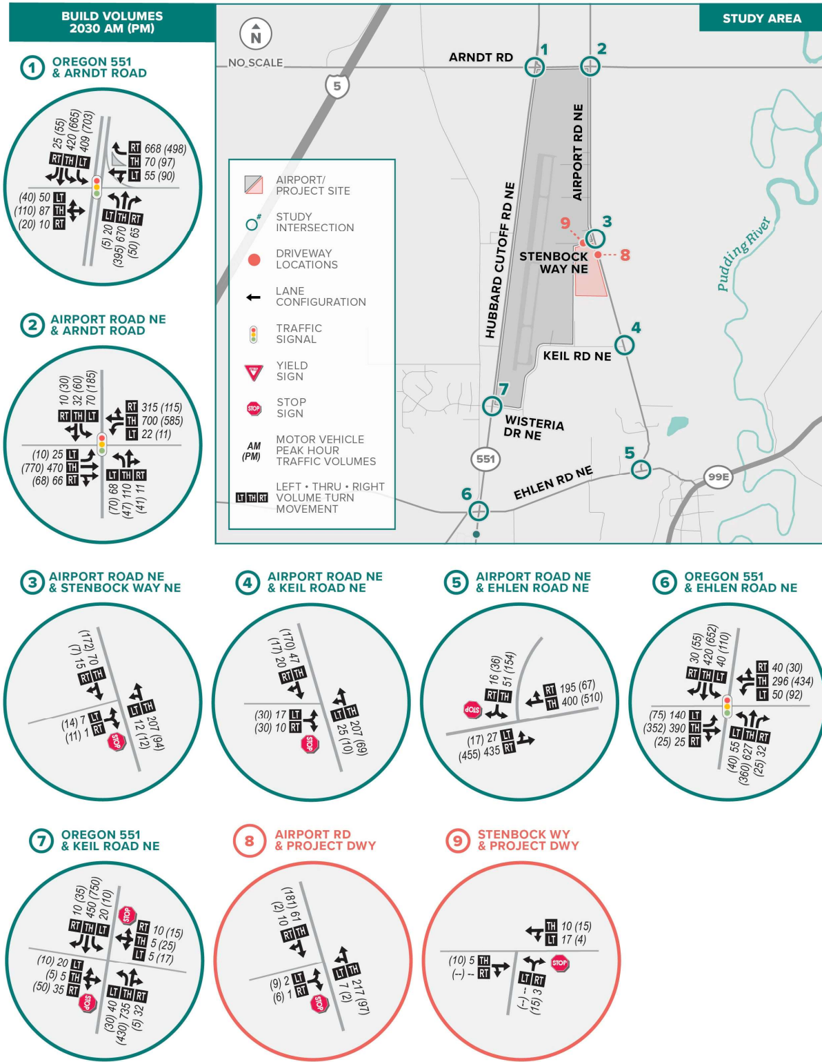
FIGURE 8: 2030 BUILD TRAFFIC VOLUMES
